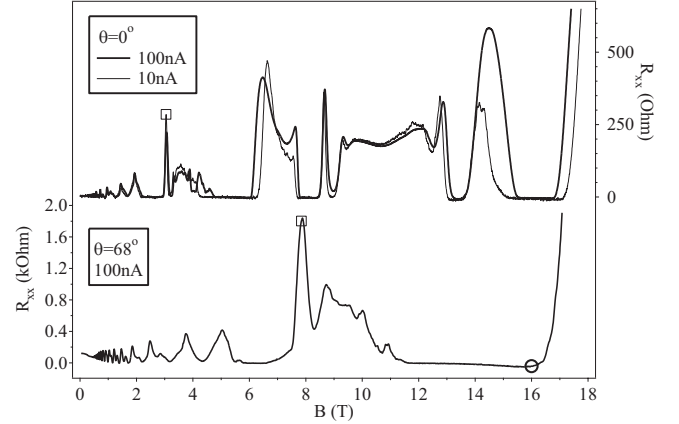
FIG. 1. Longitudinal magnetoresistance traces acquired at \theta=0^\circ (top), where \nu=1 occurs at 5.25 T and in the tilted field with \theta=68^\circ , where \nu=1 occurs at 13.9 T. In the \theta=0^\circ orientation, R_{xx} was measured using two different excitation currents: 10 and 100 nA. The bath temperature was maintained at or below \sim 20 mK. The circle on the lower trace indicates the location at which the spectrum in Fig. 2(c) was recorded.
